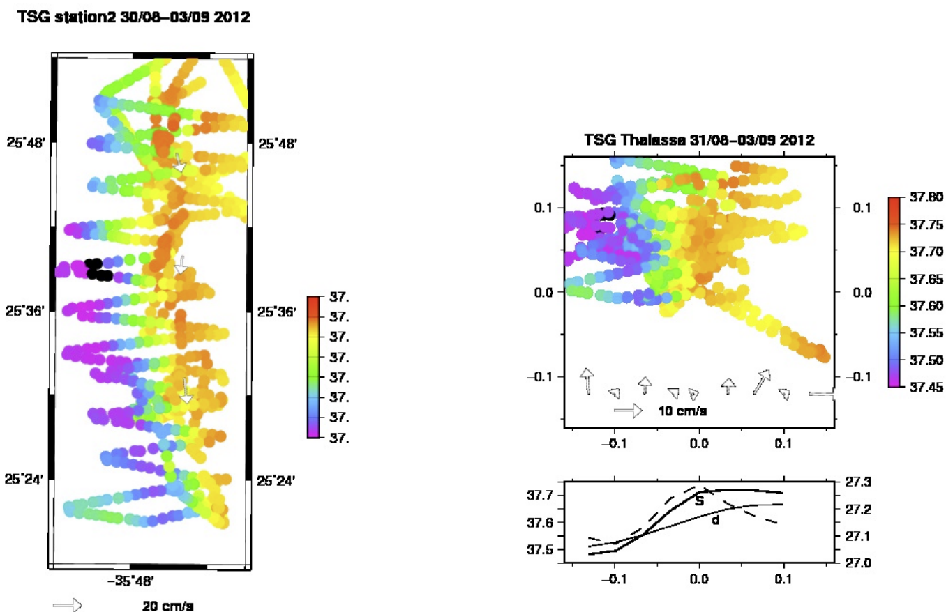
Figure 2: One of the long station surveys centered on the deployment of 5 drifters drogued at 15 m depth. Left panel, the salinity survey during the over-three days of station following the drifters. Right top panel, salinity survey (RV Thalassa TSG) in the position framework relative to the barycenter of the drifters (0.1 is 10 km). It illustrates a mostly North-South oriented filament centered at the barycenter longitude. Velocity is 15m ship-ADCP velocity relative to the barycenter motion (it shows that the filament core coincides with a maximum southward velocity). Lower panel, average night-time profiles of SST, SSS and surface density across the salinity filament.
