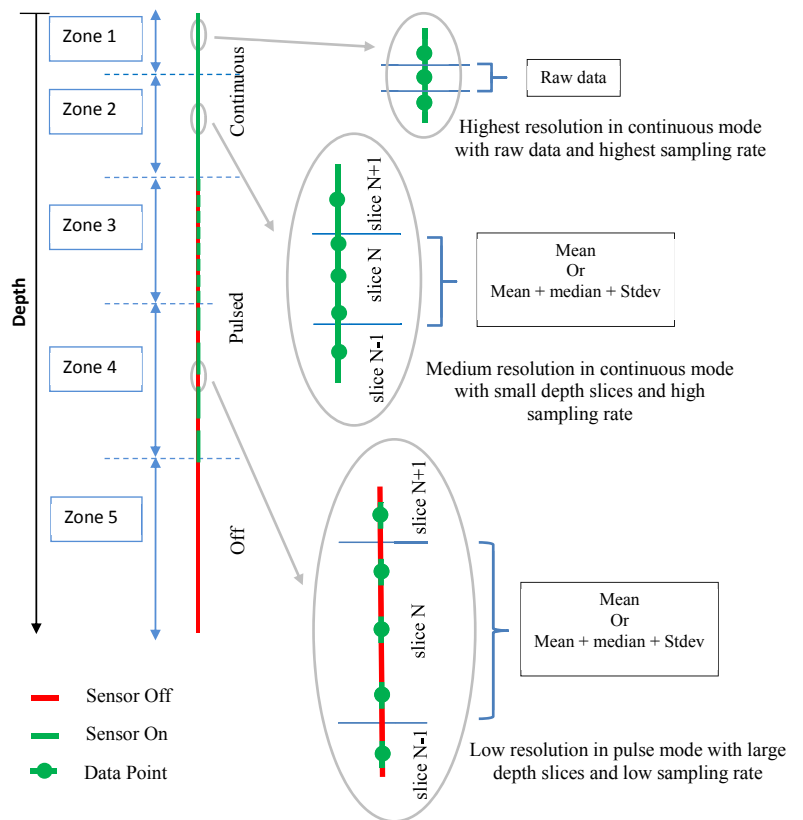
Figure 2: Sensor powering and data acquisition options along a profile. The ProvBioII float allows balancing power consumption and data resolution by controlling the sensor power supply, the sampling rate and the thickness of slices within which data will be processed. These parameters could be defined independently for each sensor for five depth intervals (Zones). In addition, within each zone, different sampling rates for descent, parking or ascent phases could be defined. This allows to have for example no (or low resolution) acquisition during the descent and the requested acquisition during the ascent of the float.
