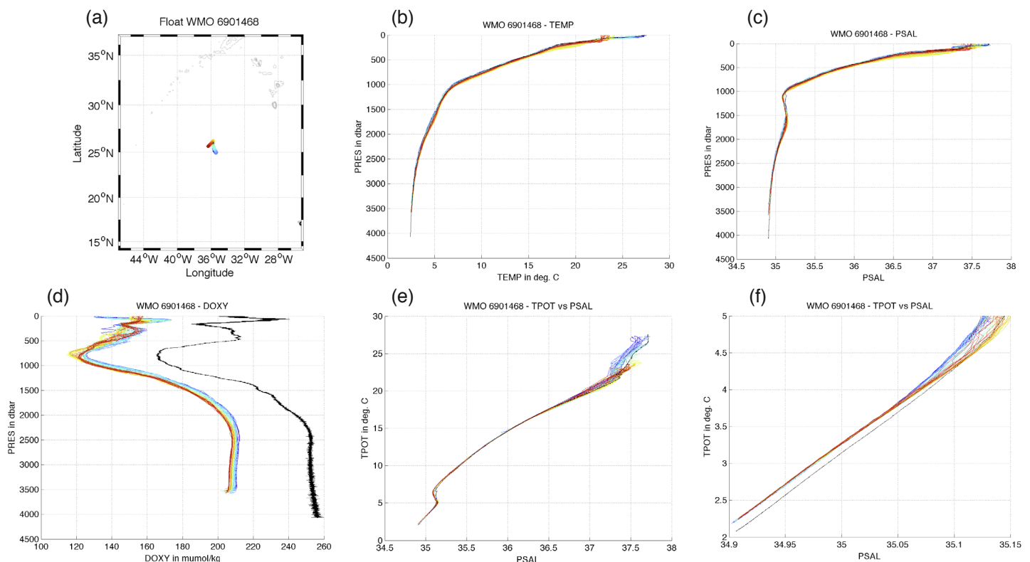
Figure 3: (a) Profiles position of the deep Arvor deployed during the Strasse cruise. (b, c, d) Temperature, salinity and oxygen profiles (in \mu\text{mol/kg} ), respectively. (e, f) \theta/S diagram. On the figures, the colored curves, from blue to red, are relative to time since deployment. The black curves are the calibrated CTD data acquired at the float deployment
