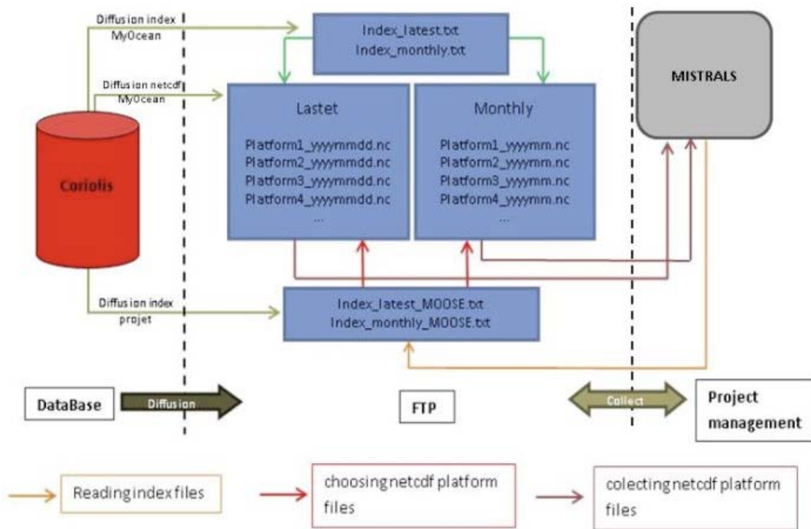
Figure 8: Customization for Moose purposes
