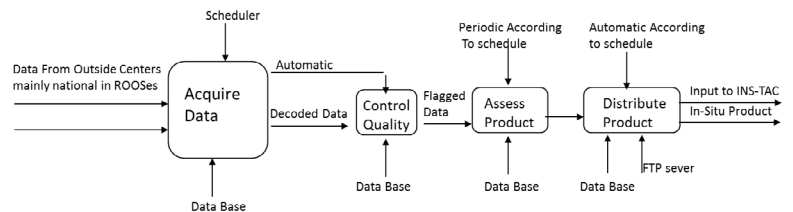
Figure 2: Functions to be implemented by an in-situ TAC component
