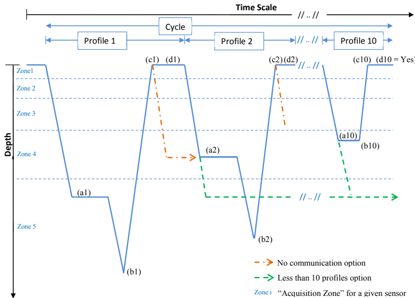
Figure 1: Navigation options of ProvBioII float: from 1 to 10 profiles could be programmed per cycle. For each profile, it is possible to define: (a) parking depth, (b) starting profile depth, (c) time schedule for surface (over several days), (d) Positioning and communication option (Yes or No). Five "Acquisition Zones" could be defined for each sensor within which acquisition parameters could be personalized.
