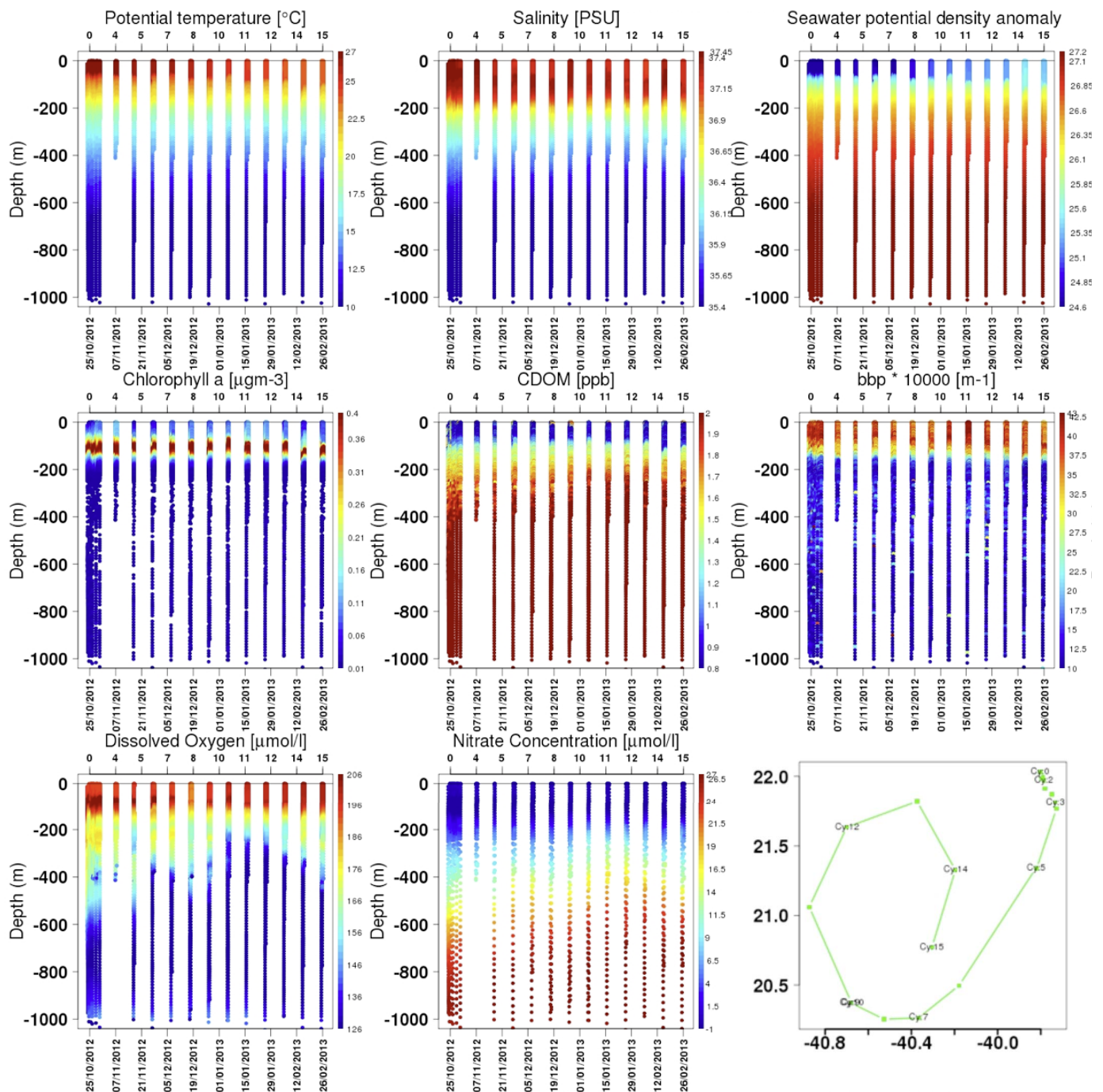
Figure 4: Data from a ProvbioII float deployed near 22°N/40°W on October 22 2012 as part of the AMT cruise. The float was programmed to acquire 4 profiles per day every 10 days. The biogeochemical payload of this float is the most complete to date and also includes transmissiometry and radiometry measurements (data not shown). Data can be seen in real time at: http://www.oao.obs-vlfr.fr/carto/
